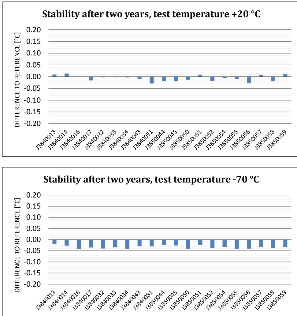
Figure 1. Stability test results of RS41 temperature measurement in two test temperatures after two years of storage. The measurement uncertainty of the test system was 0.07 °C (k=2).
