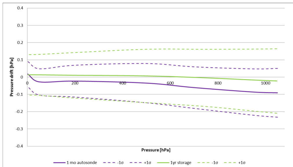
Figure 5. Mean drift in RS41-SGP pressure after one-month storage in conditions similar to those in Vaisala AUTOSONDE® (purple) and after one-year storage in radiosonde foil packaging (green).
