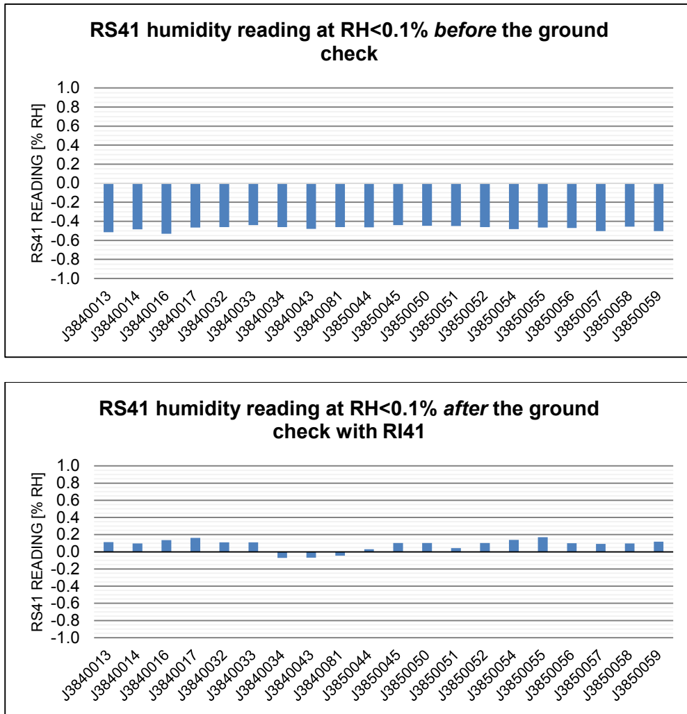
Figure 2. Stability test results of RS41 humidity measurement after two years of storage before and after ground check. The readings averaged over 30 seconds in dry conditions without ground preparation procedures (top), and with the recondition heating and zero humidity check applied, dry conditions (bottom). The humidity level at the dry test condition was below 0.1 % RH.
