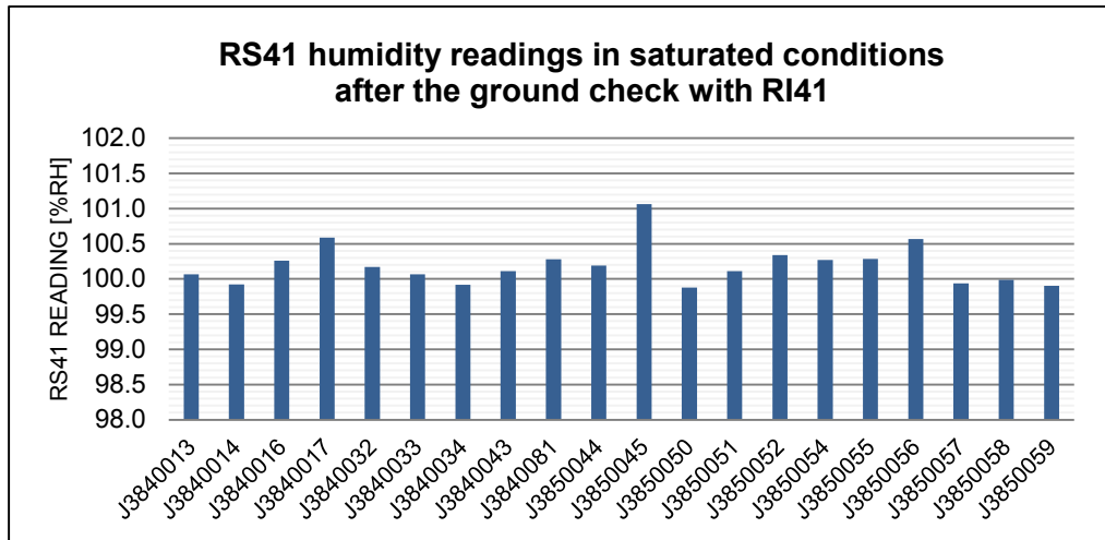
Figure 3. Stability test results of RS41 humidity measurement after two years of storage in saturated conditions after ground check. The readings averaged over 30 seconds. The saturated condition was generated with a Standard Humidity Chamber.
